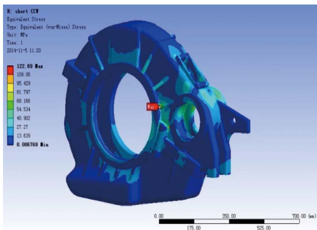
FEA of main elements
